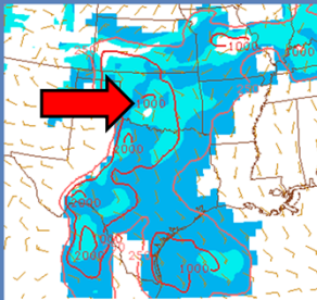
MLCAPE: 1000 j/kg
