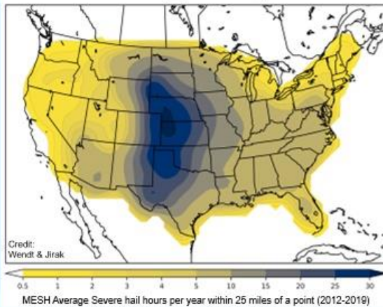
Severe ( \geq 1 -inch) Hail
