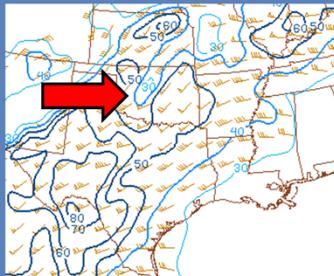
0-6 km shear: 30-50 kt
